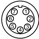
712 Binder Connector 7c - male pinout solder view
