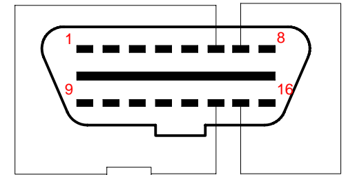
OBD II 16c connector pinout solder view
