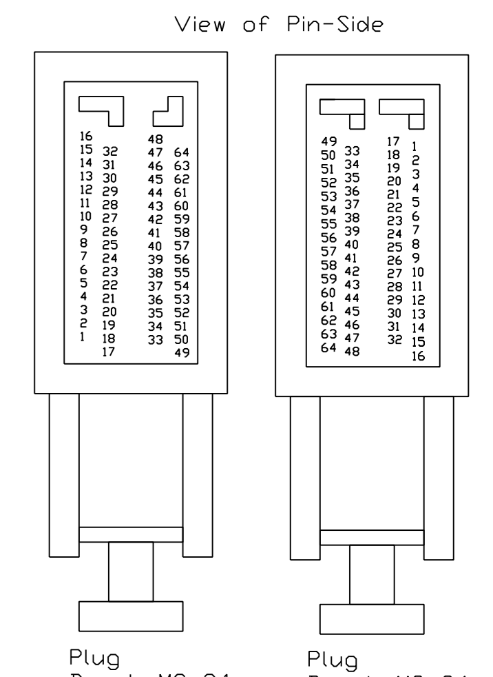
View of Pin-Side Plug Bosch MS 3.1 Engine Plug 1 928 403 513 Plug Bosch MS 3.1 Chassis Plug 1 928 403 386
