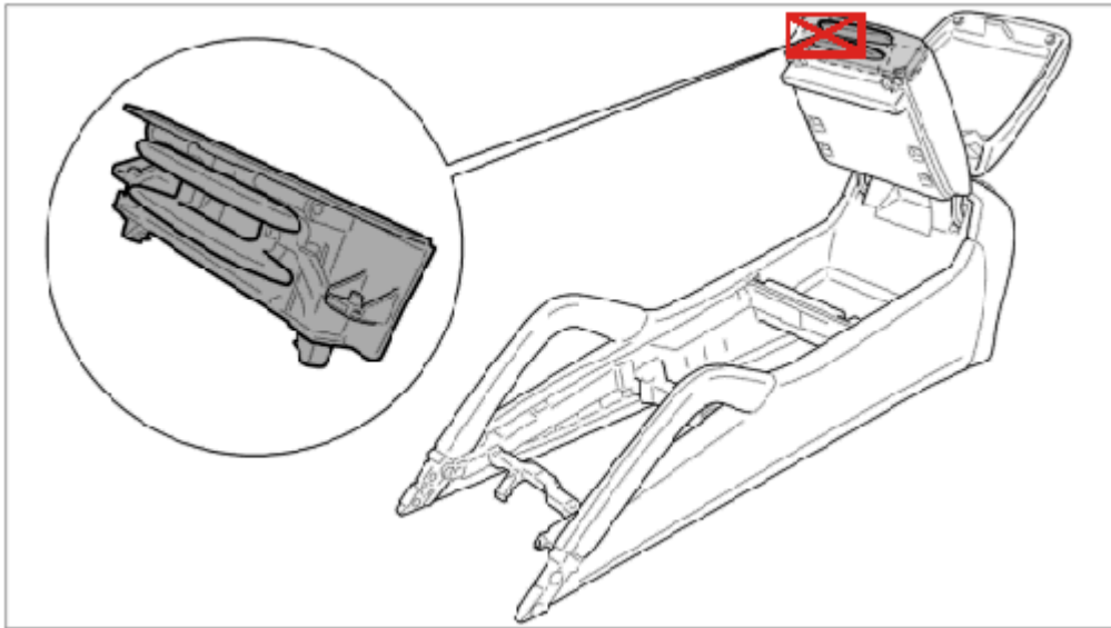
Fig. 94: Removing and installing armrest release
