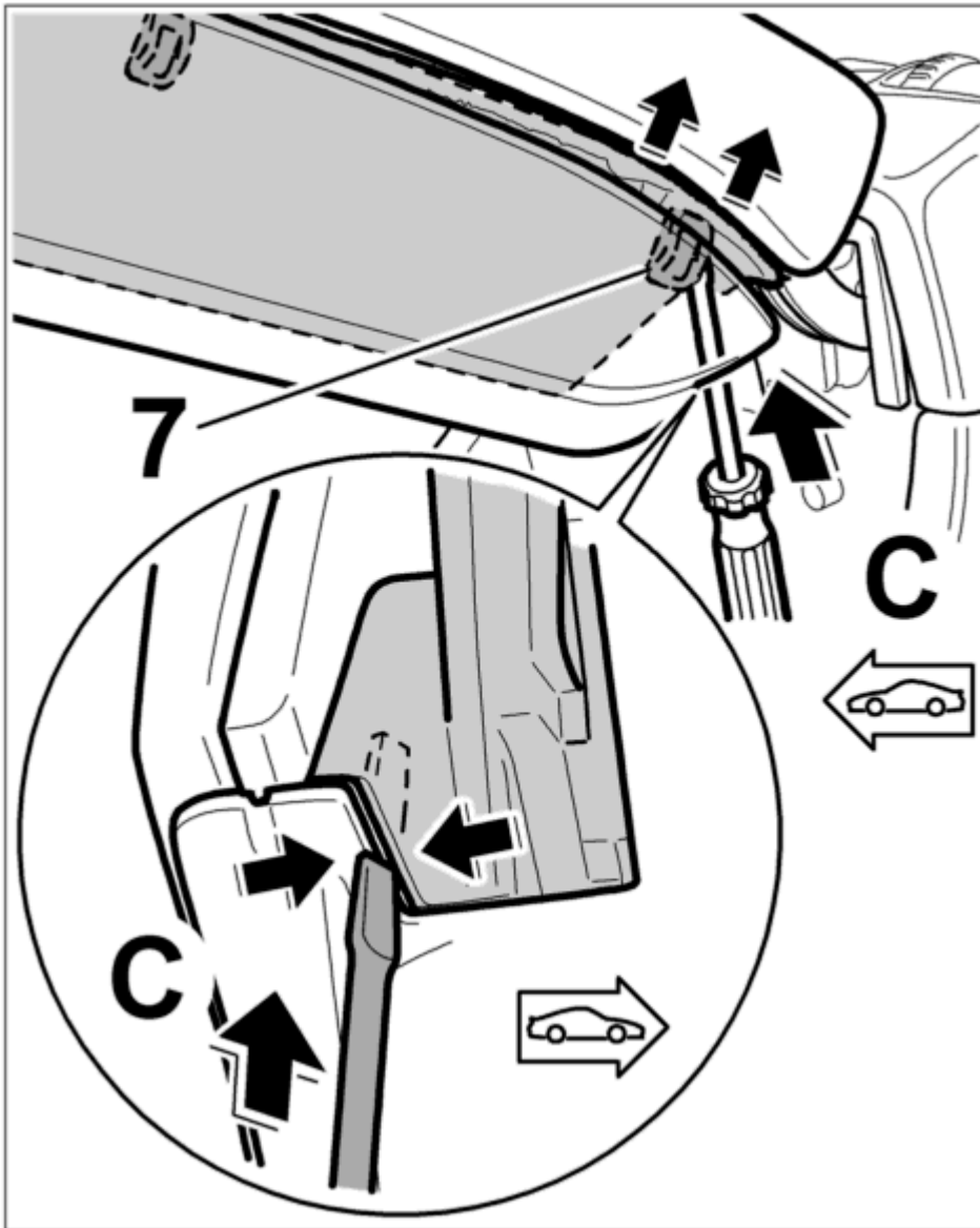
Fig. 102: Unclipping shelf
