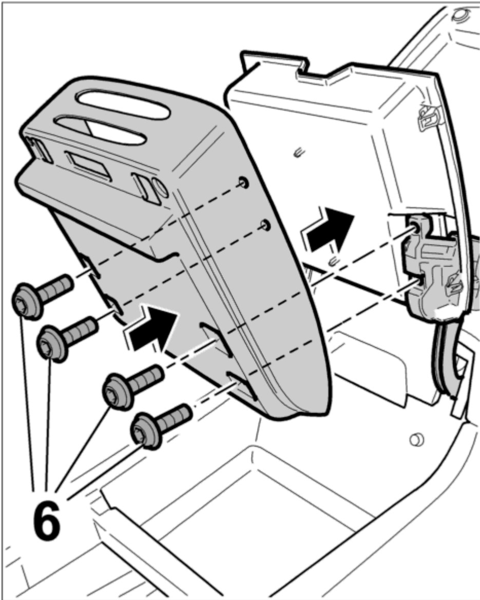
Fig. 106: Installing bottom half
