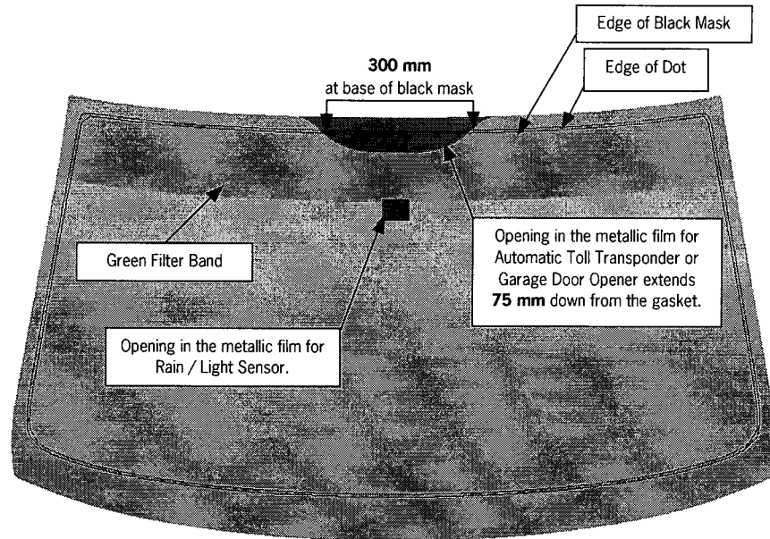
Figure 1 Cayenne Optional Thermally Insulated Glass
