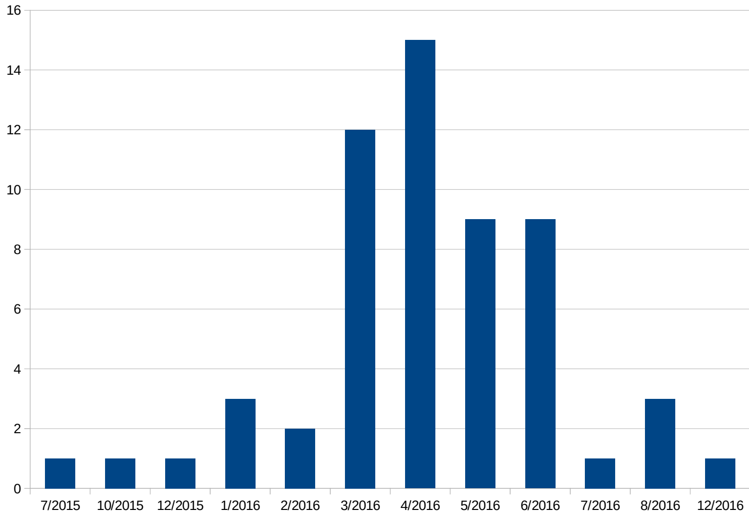
Counts of "Month of Build" for 3rd gear Failures
