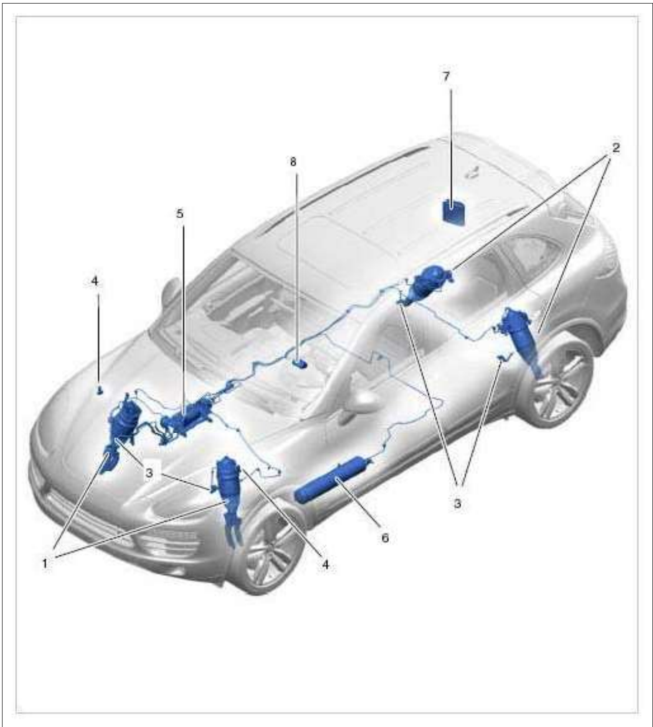
Fig 1: Overview Of Air Suspension System Component Arrangement
