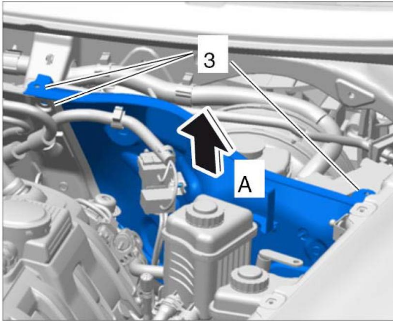
Fig 4: Removing Right Cross Panel (Left)
