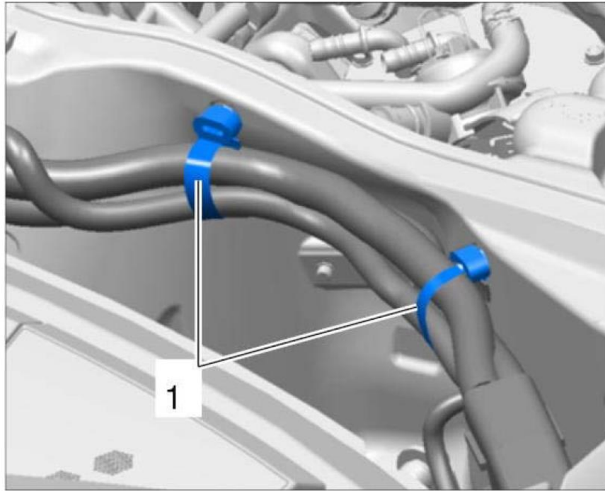
Fig 2: Identifying Tie-Wraps Wire Harness
