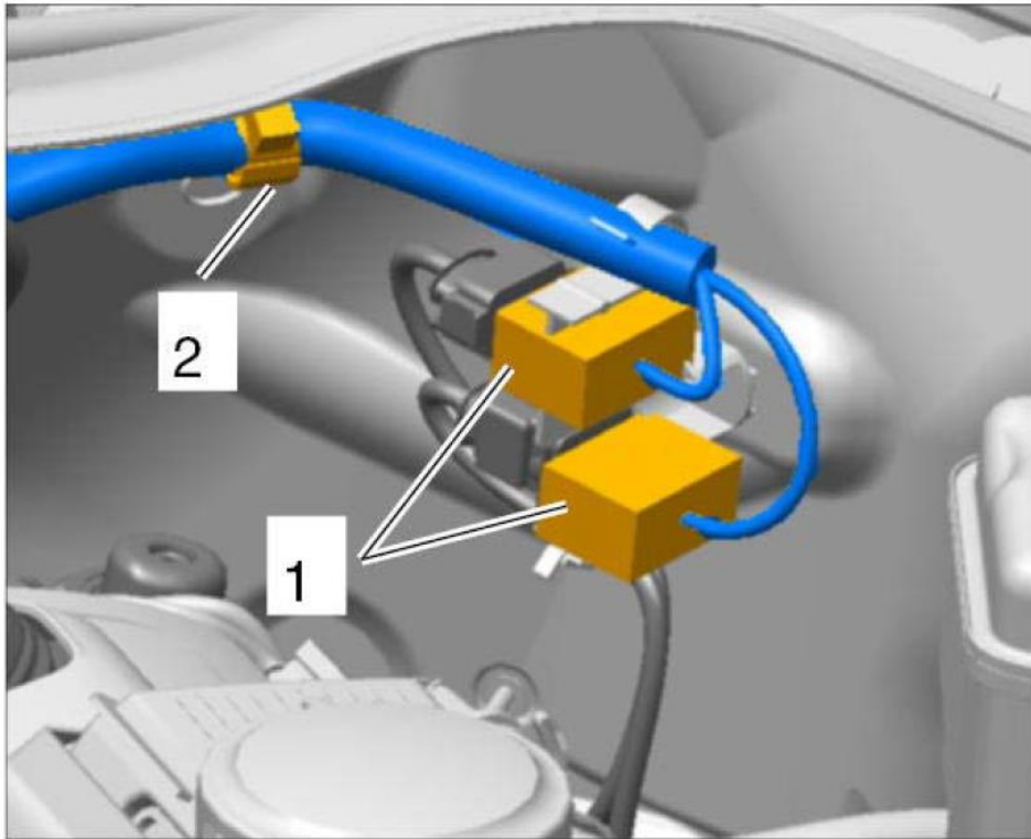
Fig 1: Identifying Plug Connections From Bracket
