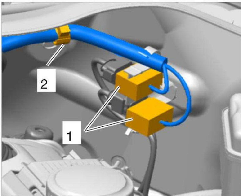
Fig 1: Identifying Plug Connections From Bracket
