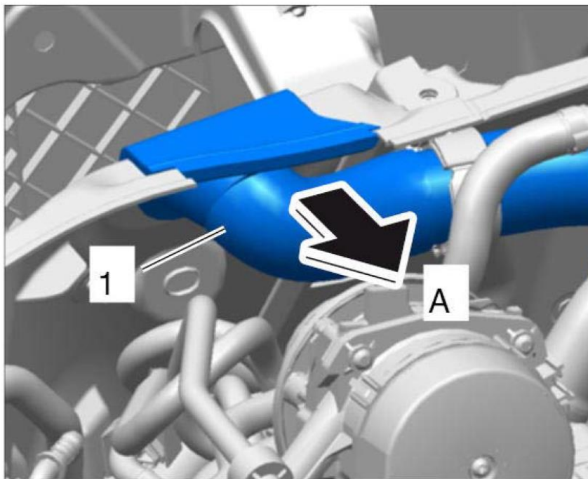
Fig 3: Removing Rubber Sleeve On Cable Bushing From Cross Panel
