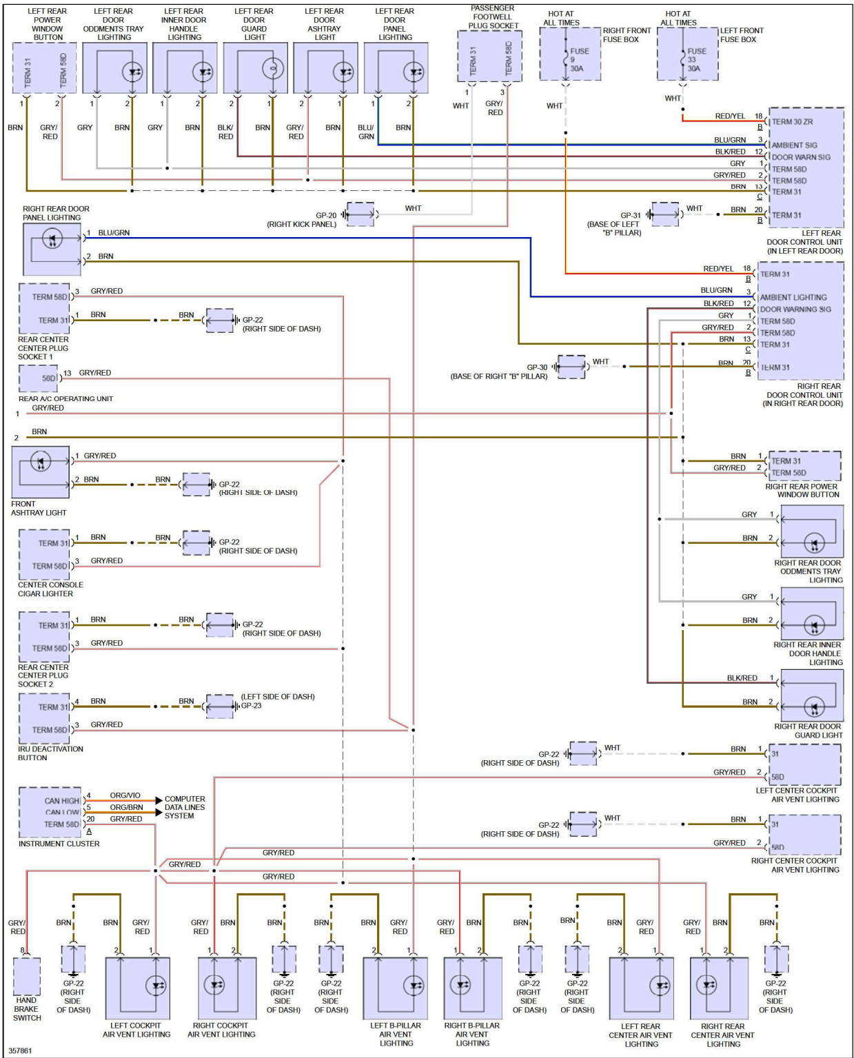
Fig 3: Interior Lights Circuit (3 of 3)
