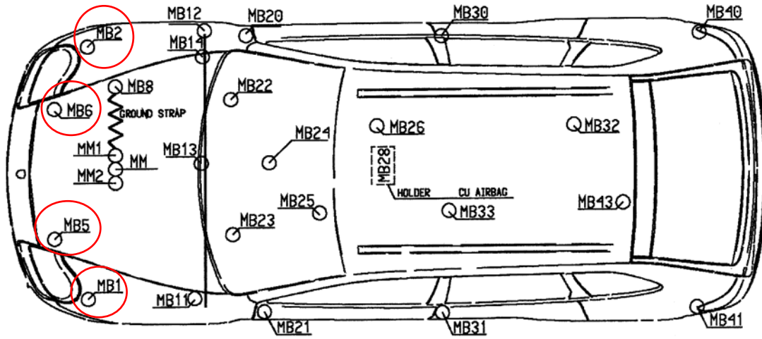
Fig. 1: Vehicle Ground Points
