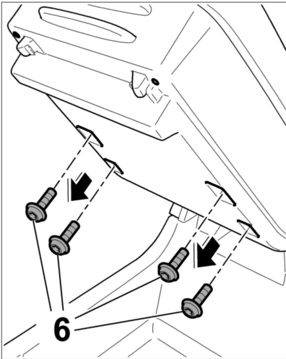
Fig. 101: Unscrewing fastening screws
