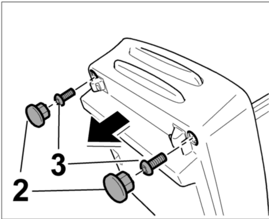
Fig. 100: Unscrewing fastening screws
