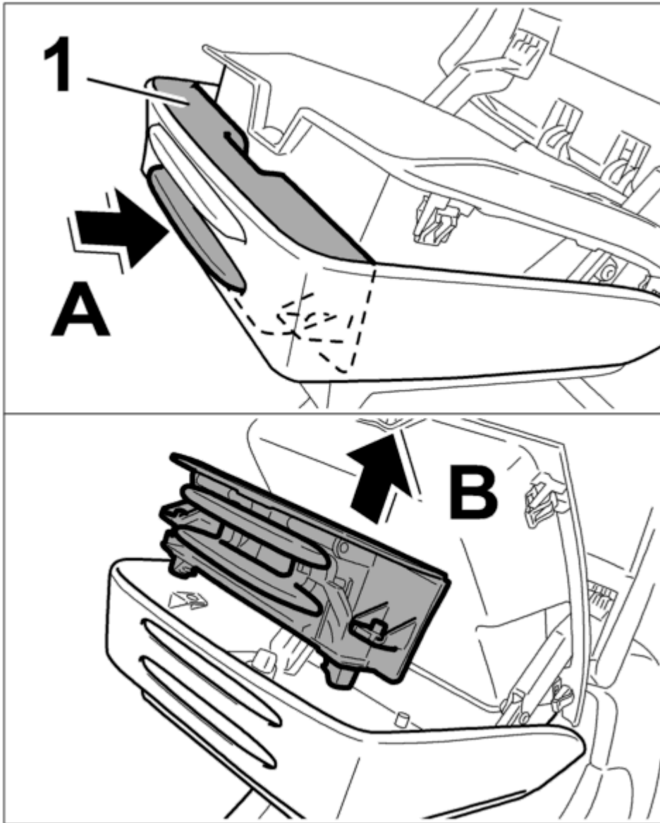
Fig. 98: Removing release
