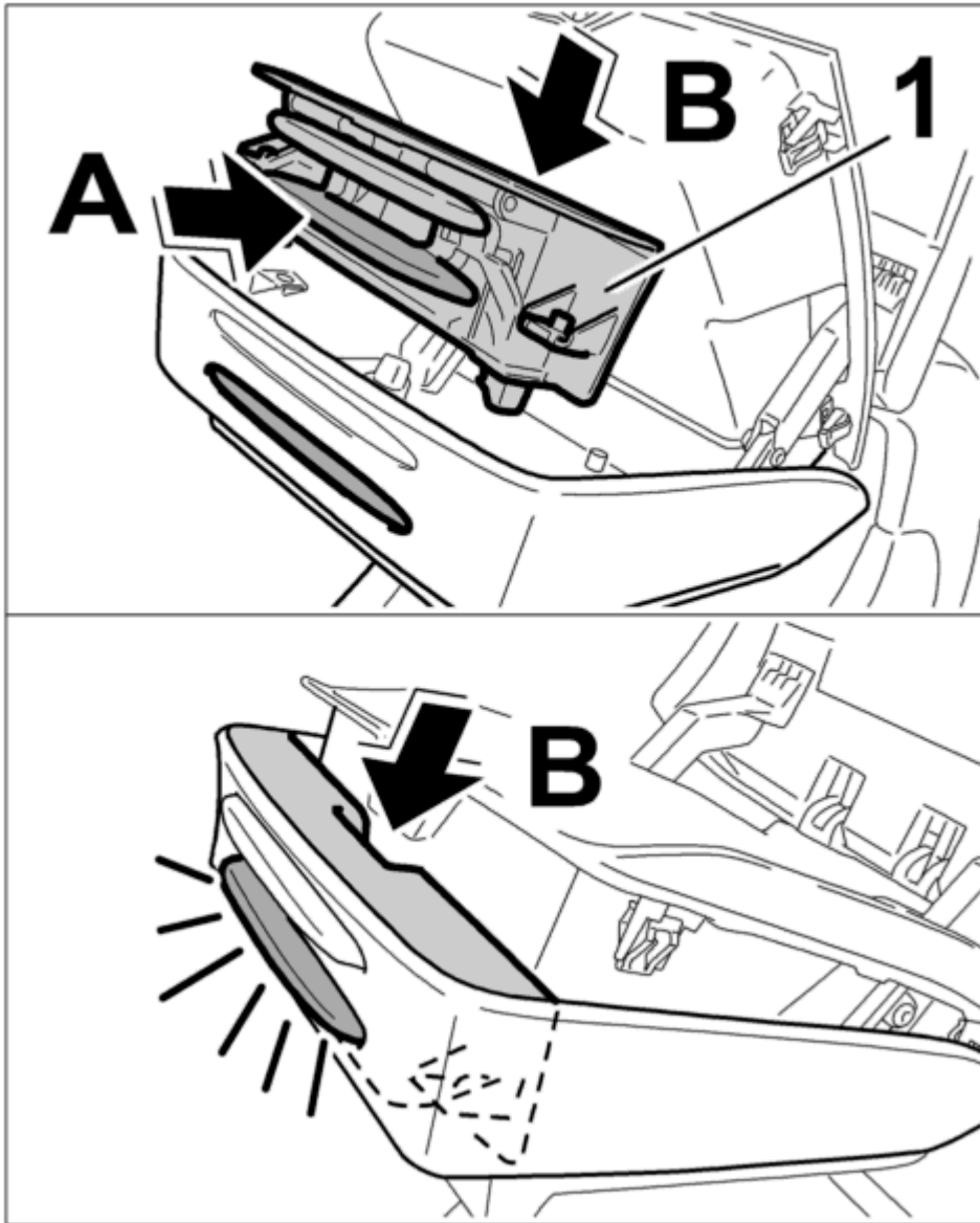
Fig. 108: Placing release in position
