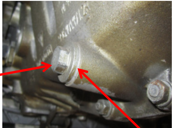
15mm bolt with aluminum crush washer
