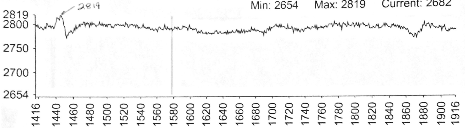
Oil Pressure, Clutch 1 (Gears 1,3,5,7,R)(bar)
