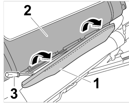
Loosening cover
