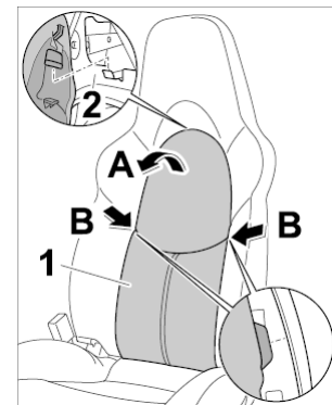
Removing cover for backrest
