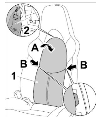
Installing cover for backrest
