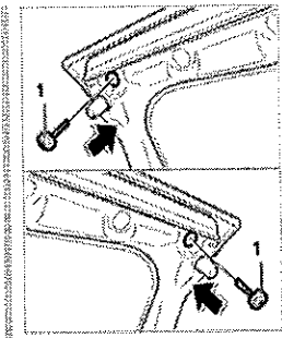
Securing reflector cover
