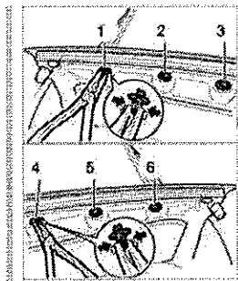
Releasing clamps
