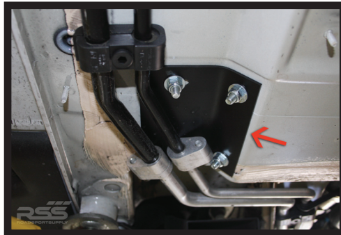
3 Holes Drilled for Underplate Installation
