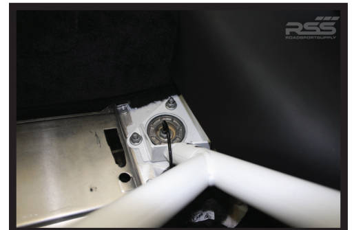
Rear Extensions Bolt To Rear Shock Towers Note: Subtle Notching of Carpet Required
