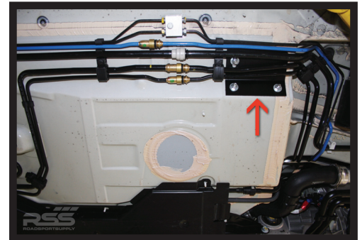
View from Under Car, Underplate Installation
