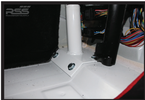
Front Legs Bolt To Floor Underneath Carpet Note: Subtle Notching of Carpet Required
