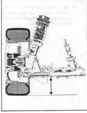
Ride Height Measurement FRONT
