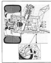
Ride Height Measurement REAR
