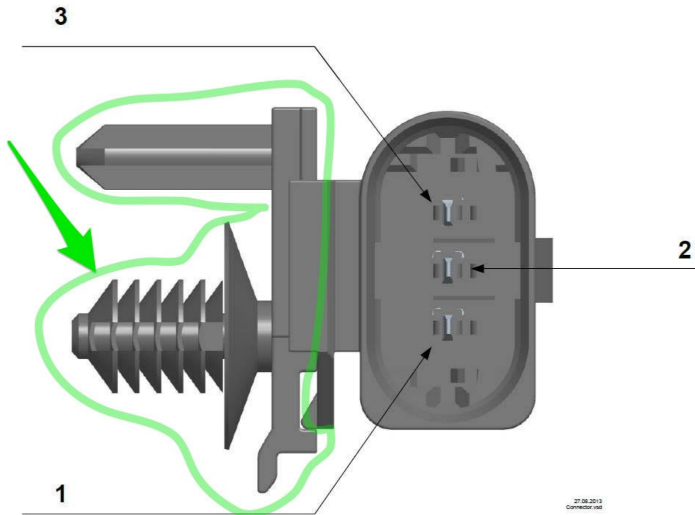
Figure 3: connector with pinout
