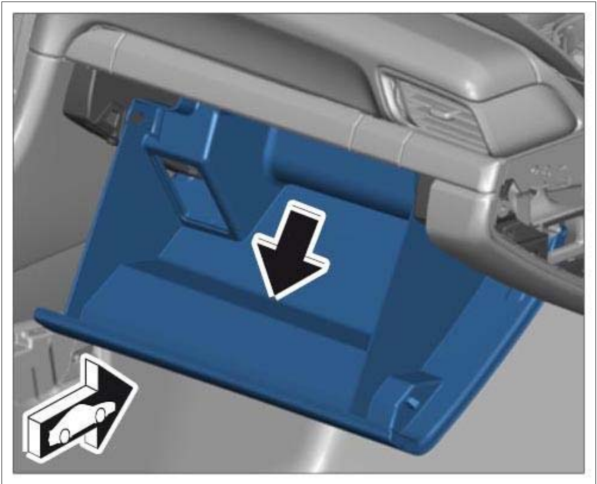
Fig 4: Unclipping Glove Compartment
