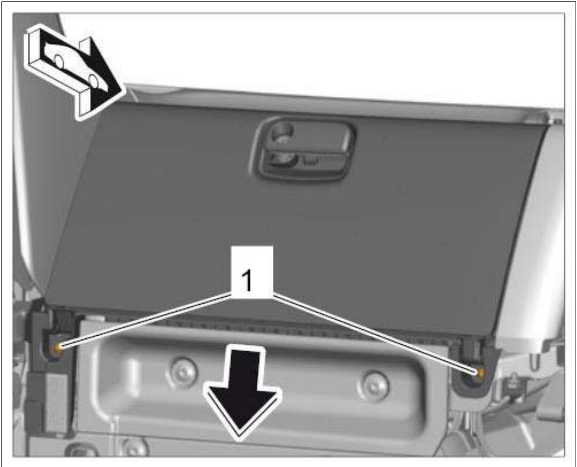
Fig 2: Loosening Mounting At Bottom
