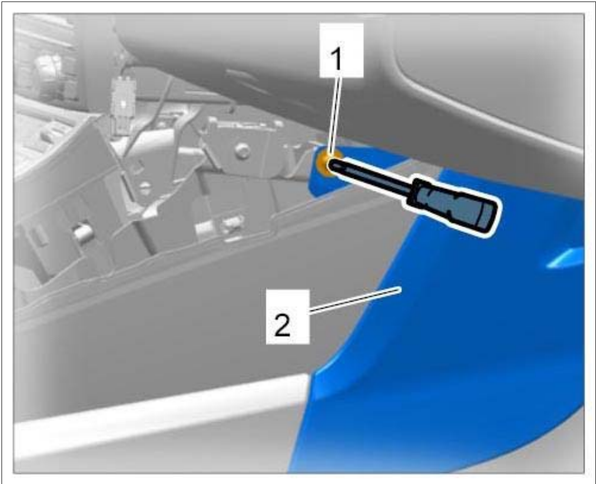
Fig 4: Detaching Footwell Outlet Vent Trim
