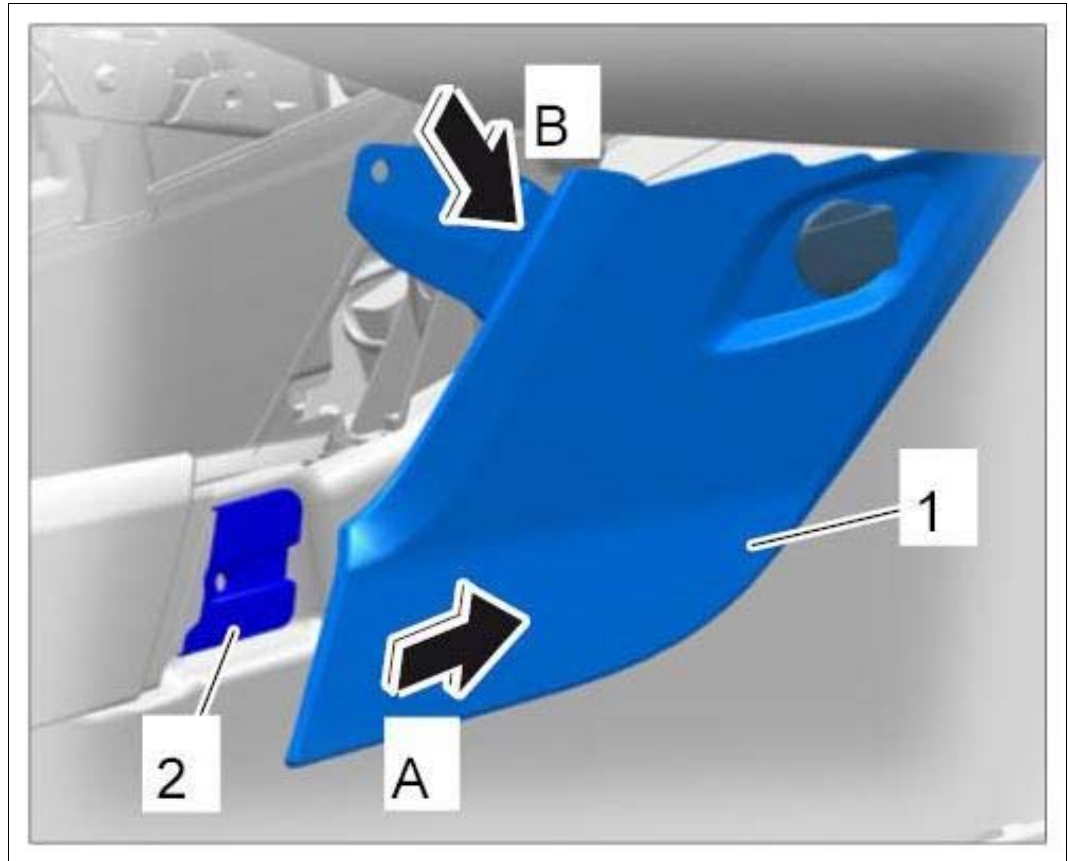
Fig 5: Removing Footwell Outlet Vent Trim
