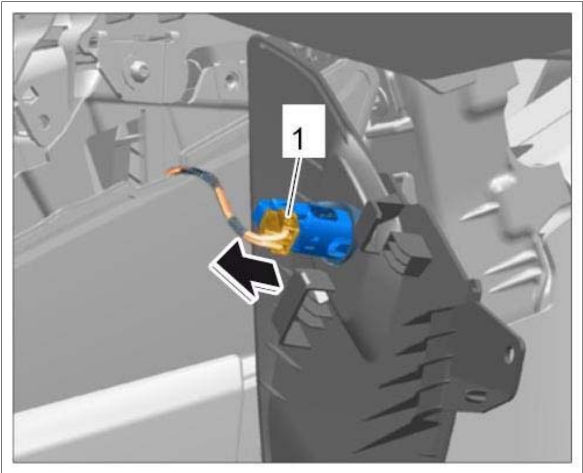
Fig 6: Disconnecting Electric Plug Connection
