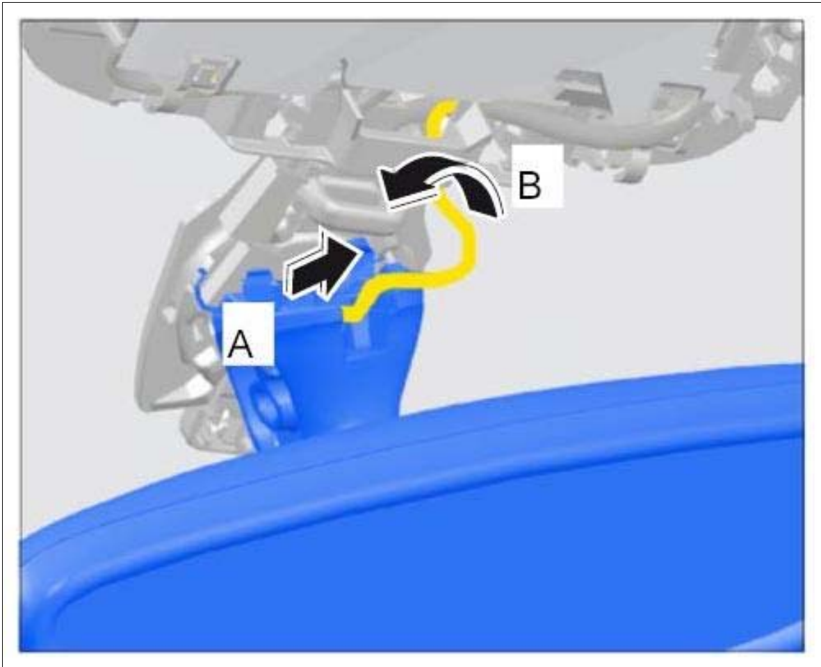
Fig 7: Removing Rear-View Mirror
