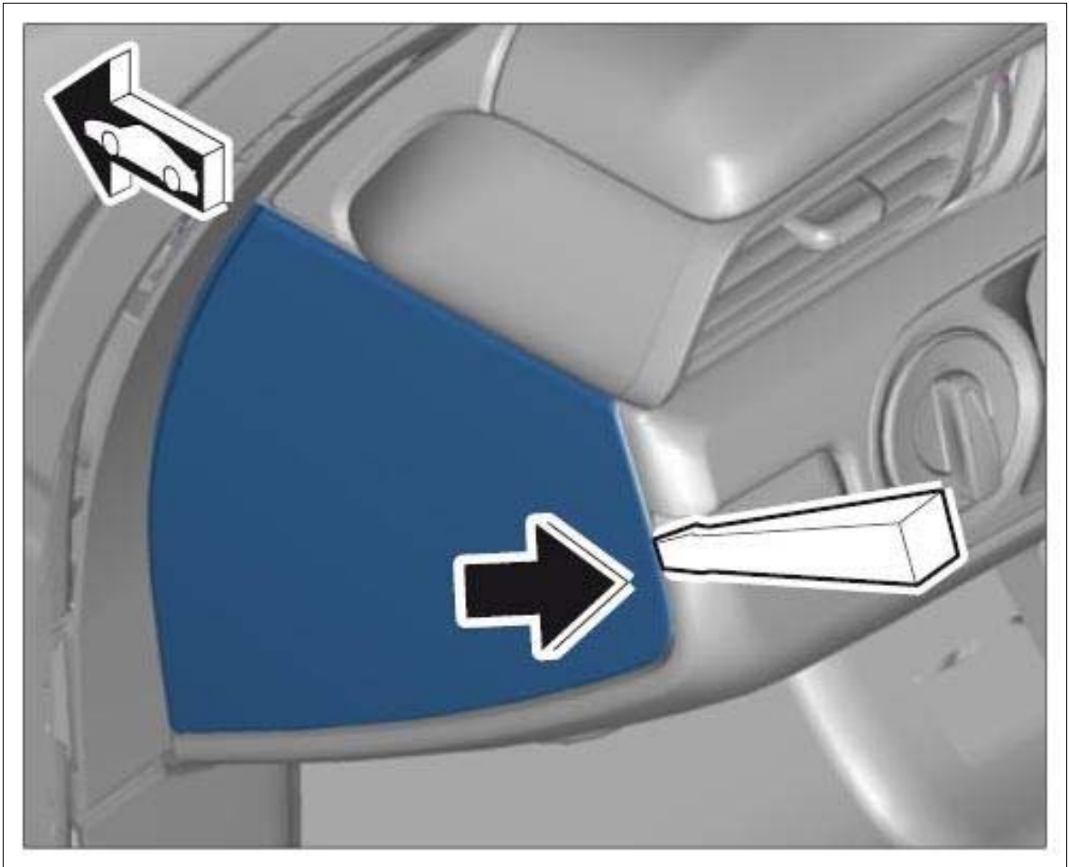
Fig 2: Removing Dashboard Trim Panel
