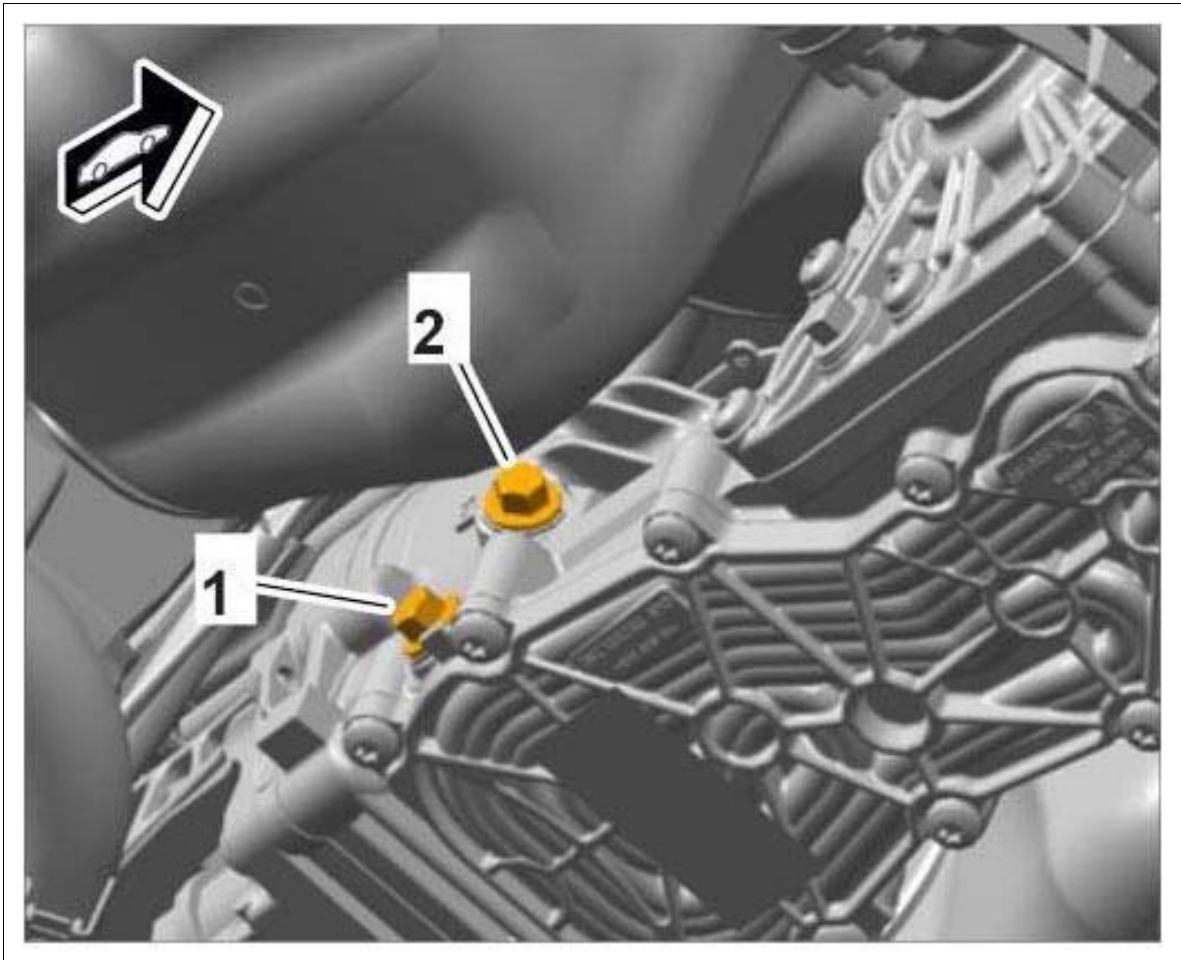
Fig 1: Removing Drain Plug And Filler Screw For Clutch Fluid
