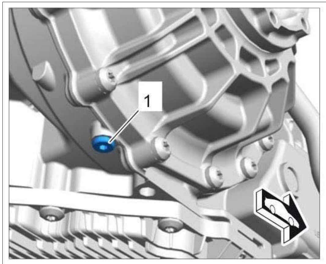
Fig 2: Removing Oil Drain Plug For Differential Space
