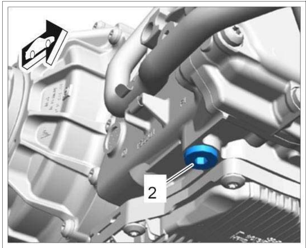
Fig 3: Removing Oil Drain Plug For Gearwheel
