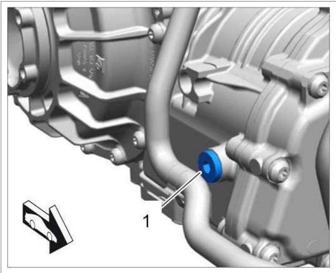
Fig 1: Removing Oil Filler Screw/Inspection Plug
