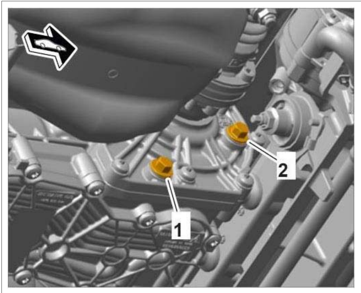
Fig 1: Identifying Drain Plug And Filler Screw For Differential Oil
