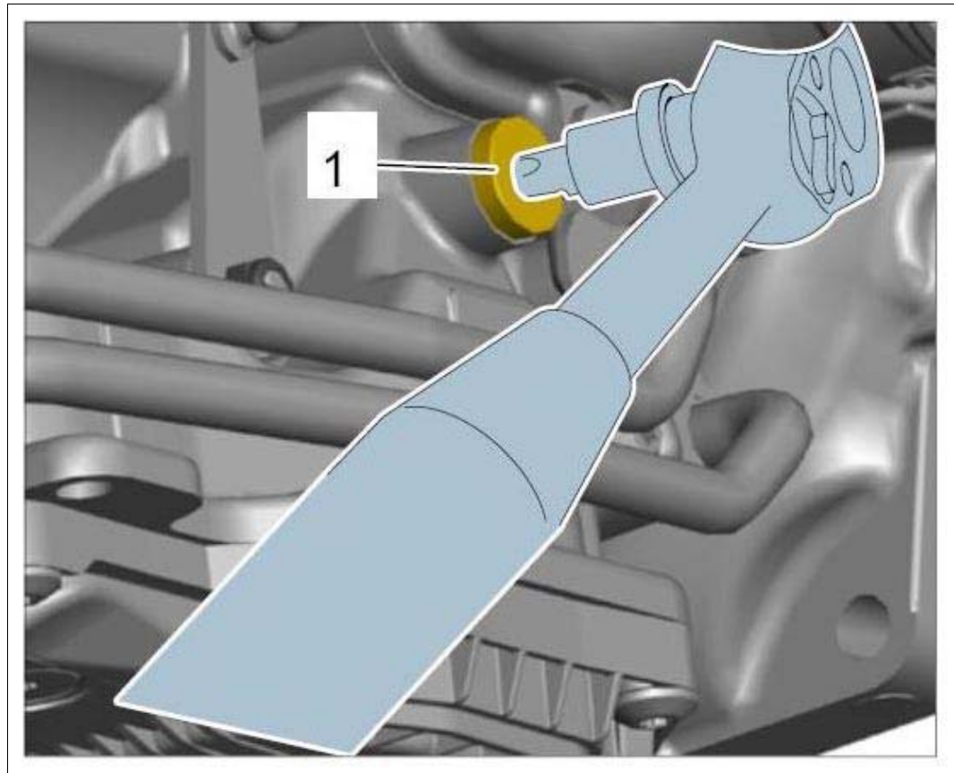
Fig 3: Tightening Oil Filler Screw
