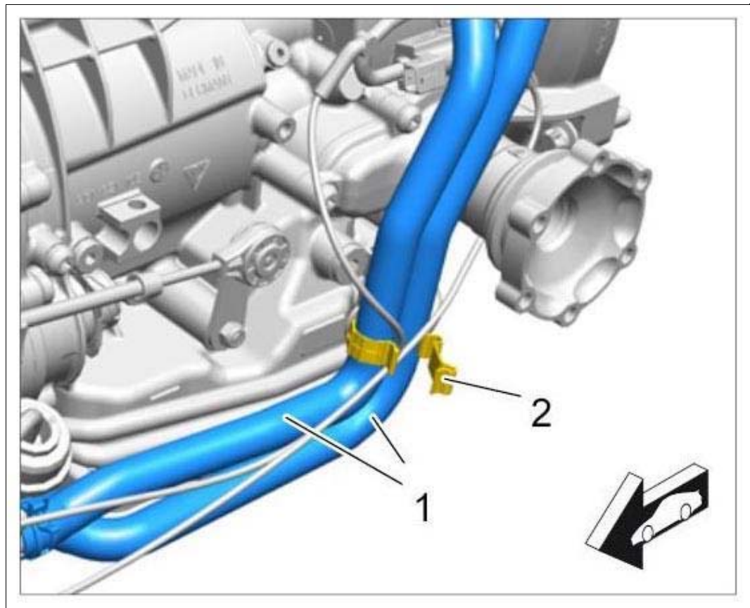
Fig 1: Loosening Coolant Hoses
