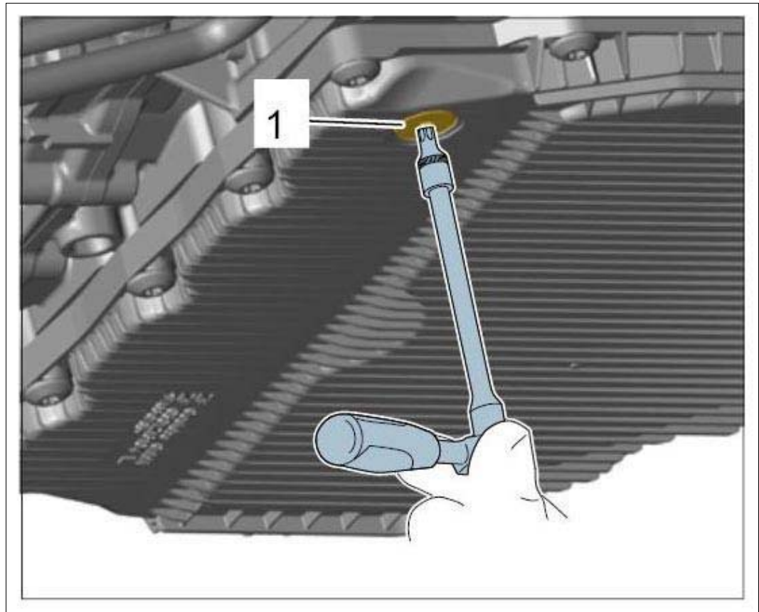
Fig 1: Identifying Drain Plug
