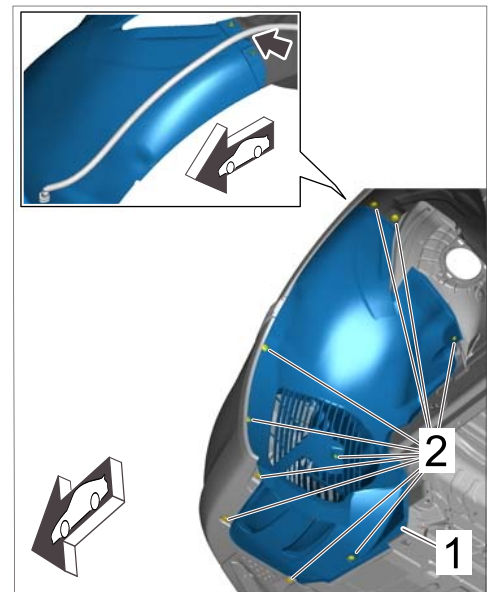
Front wheel housing liner - front part
