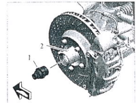
Inserting the lockable wheel bolt in the wheel hub
