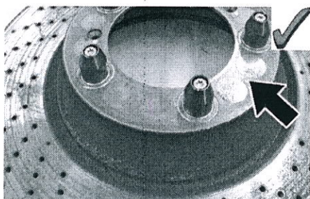
Brake disc OK
