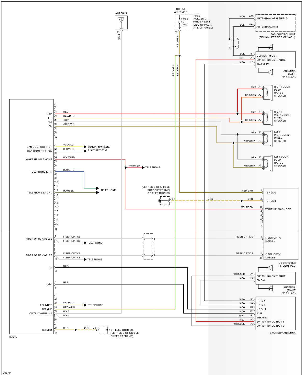
Fig. 60: Radio Circuit, W/O Bose W/O Navigation
