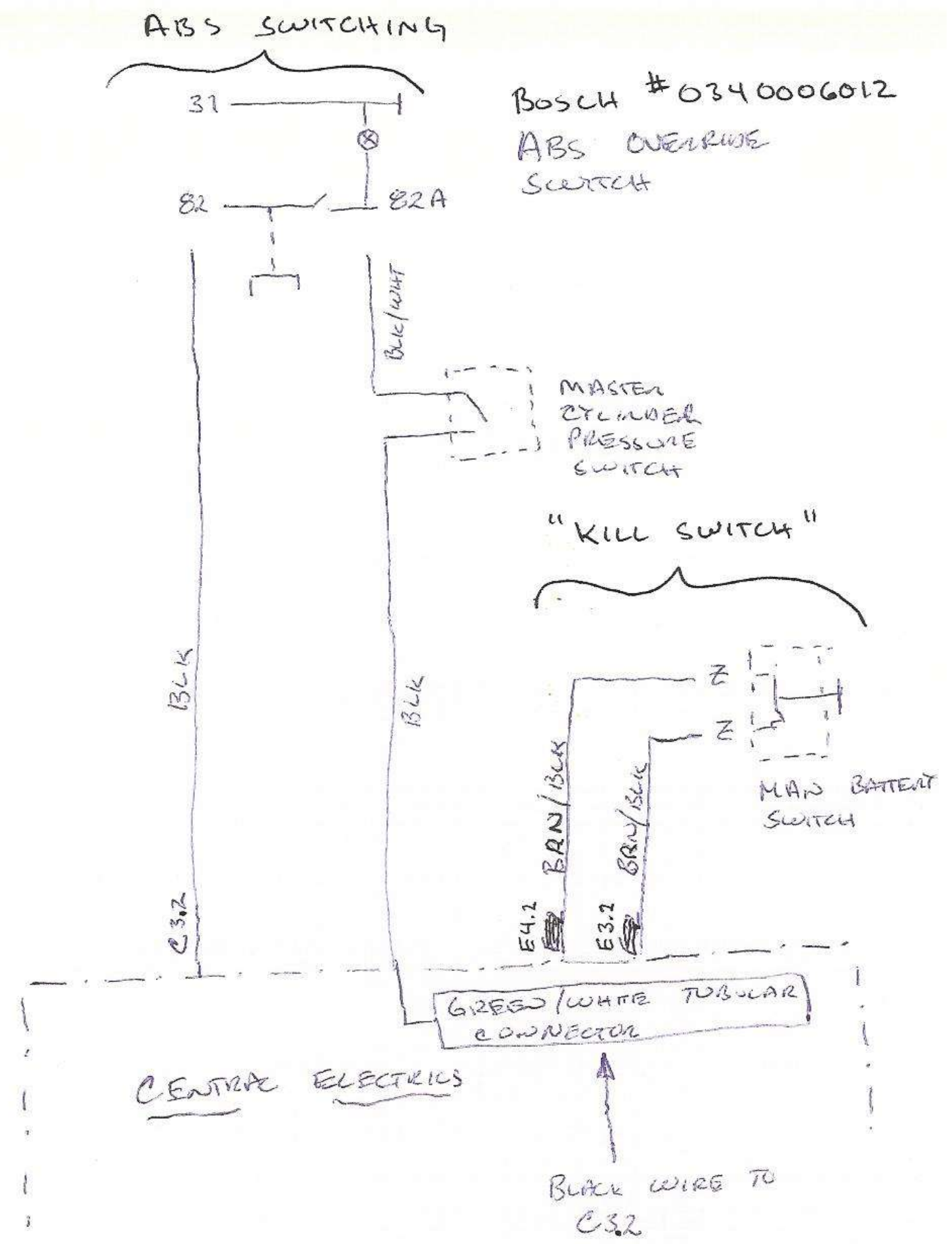
SCHEMATIC FOR CAMERA CUP ADD-ON HARNESS - ADDS EUROPEAN RS CIRCUITS TO AMERICAN C2/4 HARNESS
