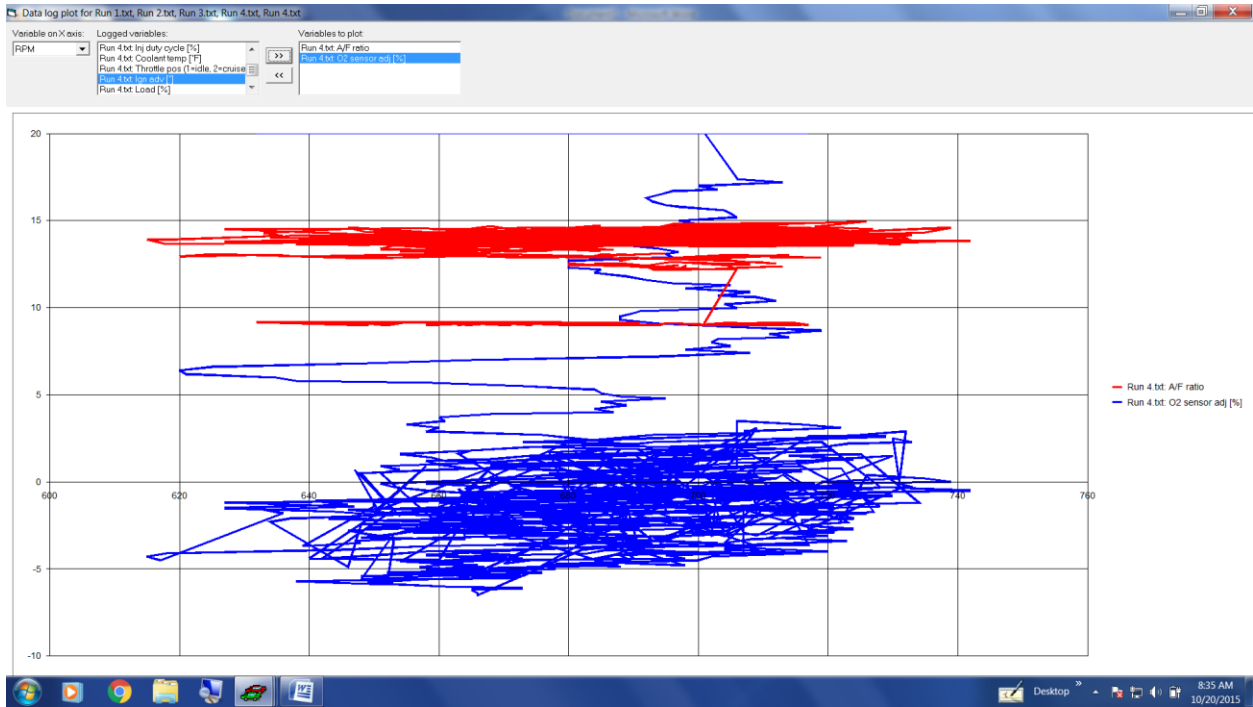
Plot 4: Same fuel map Closed loop o2 sensor adjust approx -6 to +3. Numbers make more sense but what happened to the plot format?
