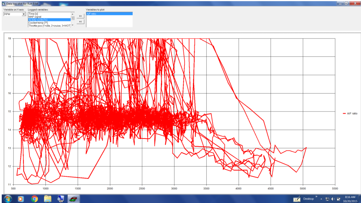
Plot 2: Same fuel map closed loop using wide band nbo2 simulator. o2 adjust approx 0-11
